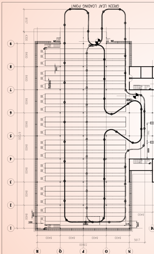
LAYOUT OF CONVENTIONAL WITHERING TROUGHS
