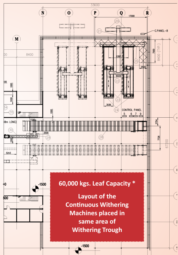
LAYOUT WITH WIZARD WITHERING MACHINES
